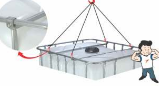
Aligned for Top Performance Top crossbars & respective verticals aligned for a box structure. Upgrades IBC for a top lift capability with reinforced cage. [Available on special request]
